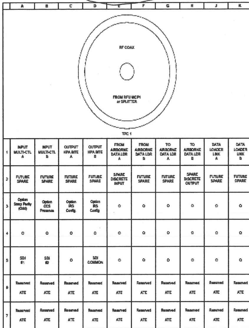
Figure 1.7-3 - External RF Block – Middle Plug Diagram (Incorrect in ARINC 771-1)
